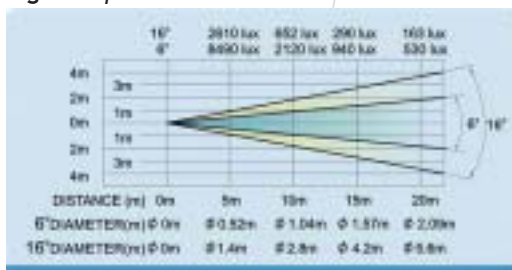
Light output chart
