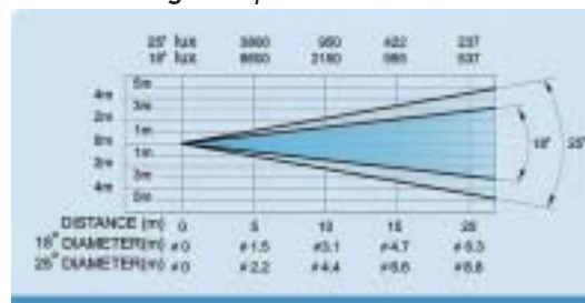
Pilot 1200 Light output chart
