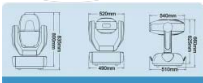
Pilot 1200 Dimensions
