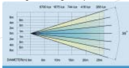
HeadLight2500 Light output chart
