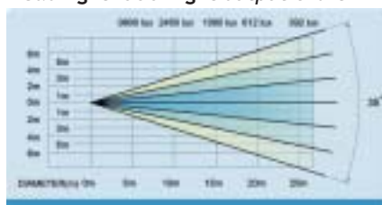
HeadLight4000 Light output chart
