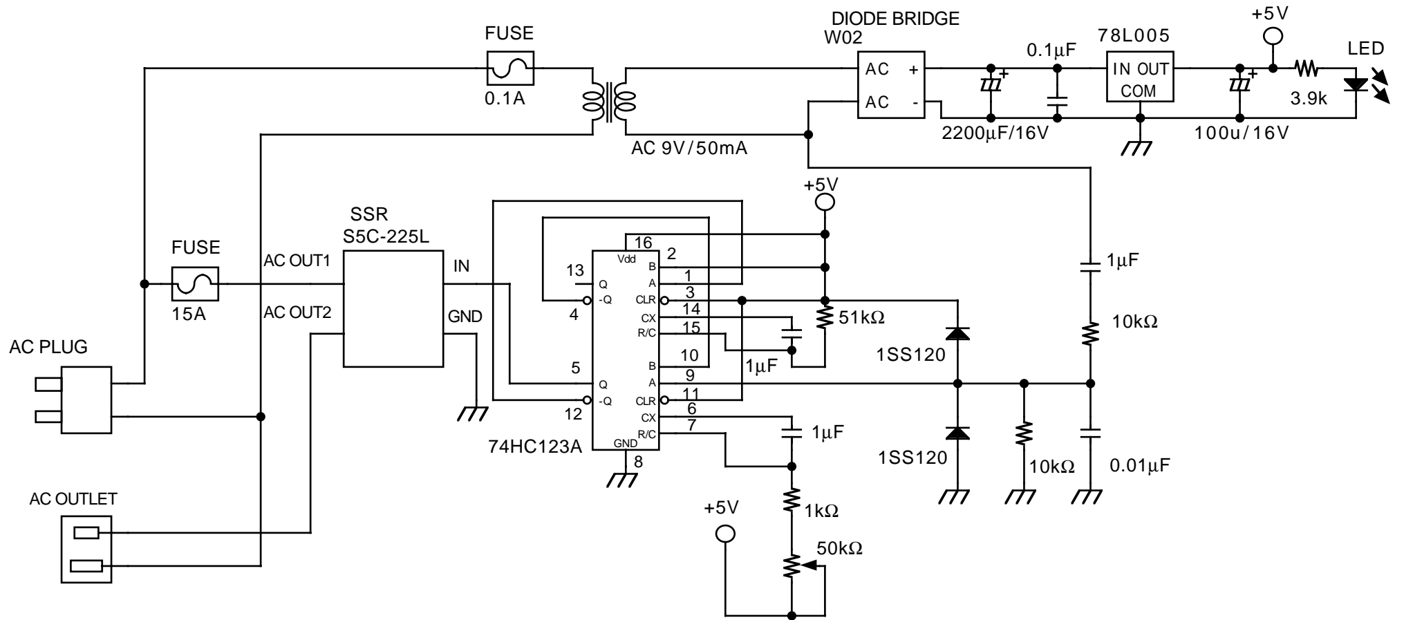
ZERO CROSS SSR AC CONTROLLER
