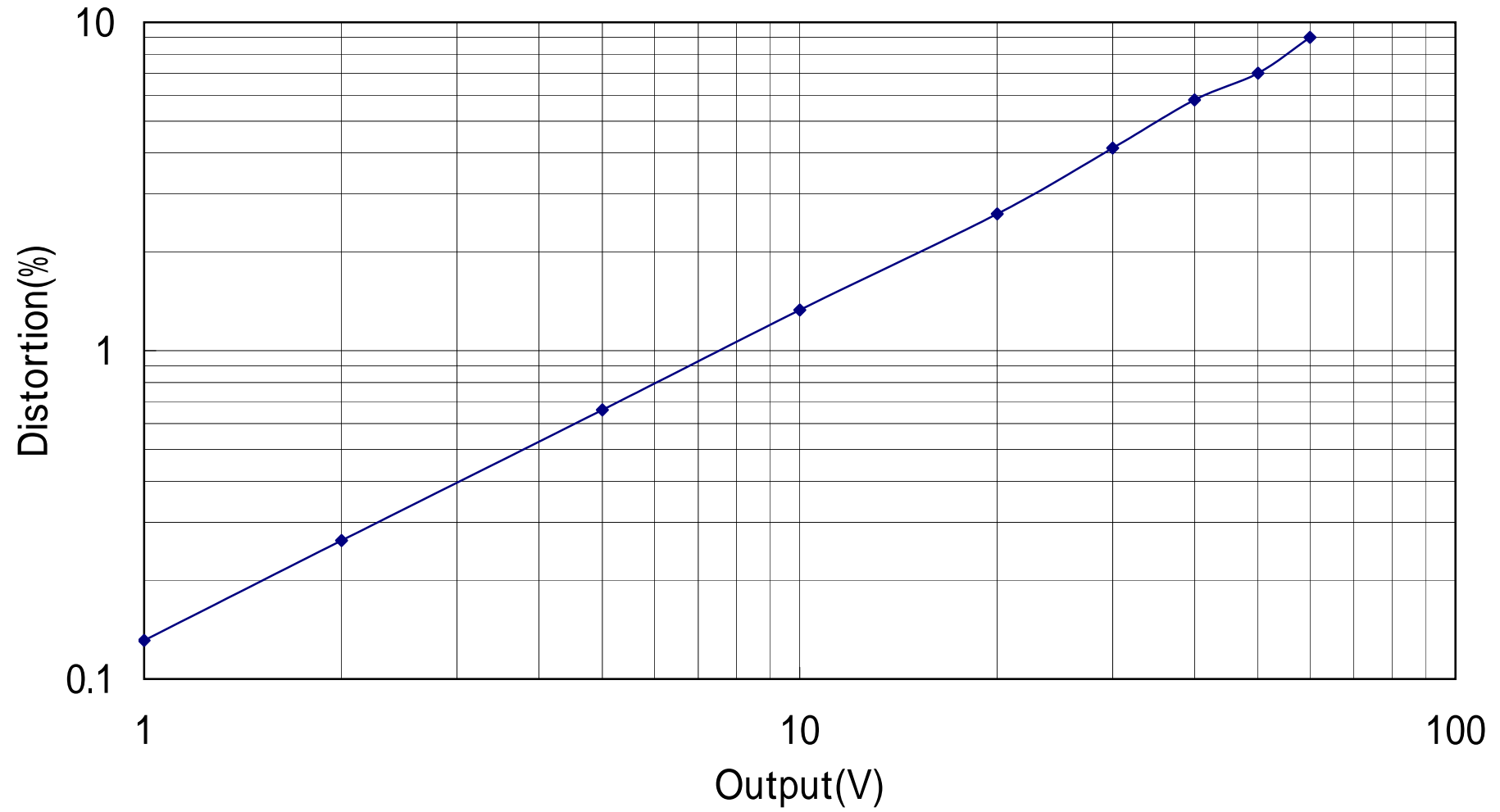
A-505(Tone Bypass)
